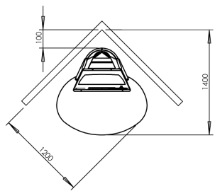
Fire Box and Flue Dimensions
